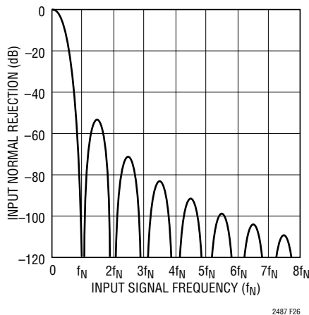
Figure 26. Input Normal Mode Rejection 2x Speed Mode
