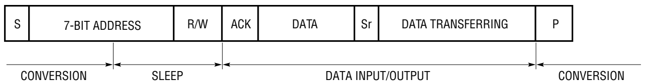
Figure 6. Conversion Sequence
