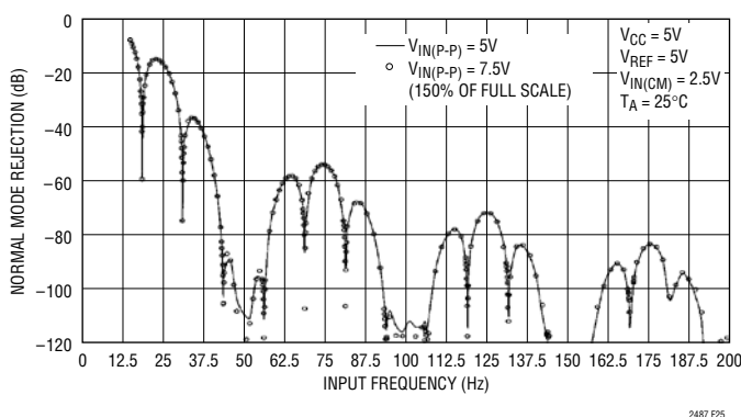
Figure 25. Measure Input Normal Mode Rejection vs Input Frequency with Input Perturbation of 150% (50Hz Notch)
